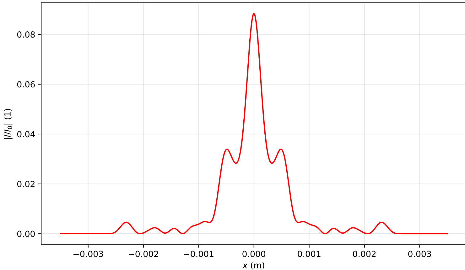
Intensity profile I(x, y = 0, z = 3.981)/I_0 , P_{in}=8.0P_{cr} , artificial time
